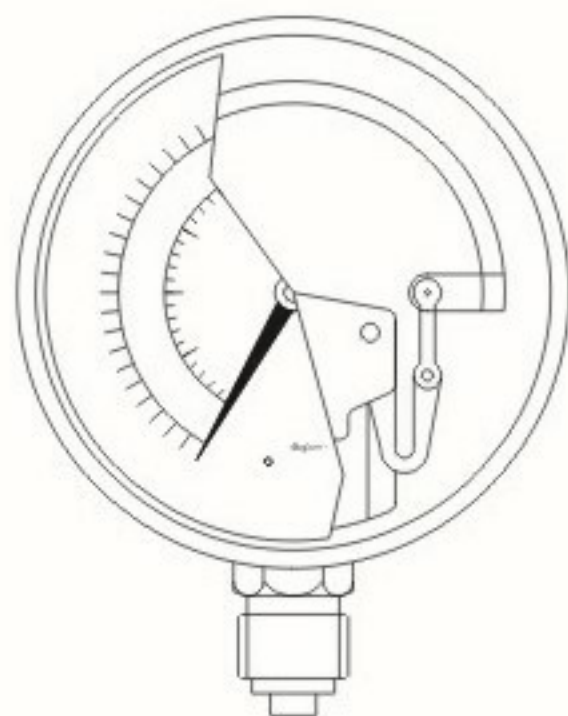
"C"-shaped Bourdon tube system
