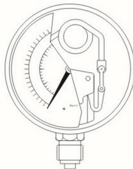
Helical Bourdon tube system
