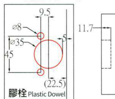
鉸杯孔 Hinge Holes
