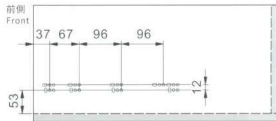
滑軌孔位示意圖 Holes Schematic
