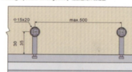
Fixing system with joint / 連接固定件孔心圖
