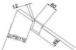
緩衝棒安裝Damper Installation
