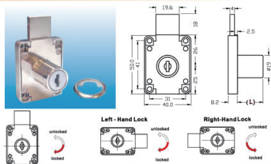
509 (22mm、30mm)
